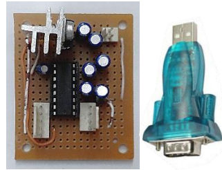
MAX232 circuit & RS232 to USB Converter
